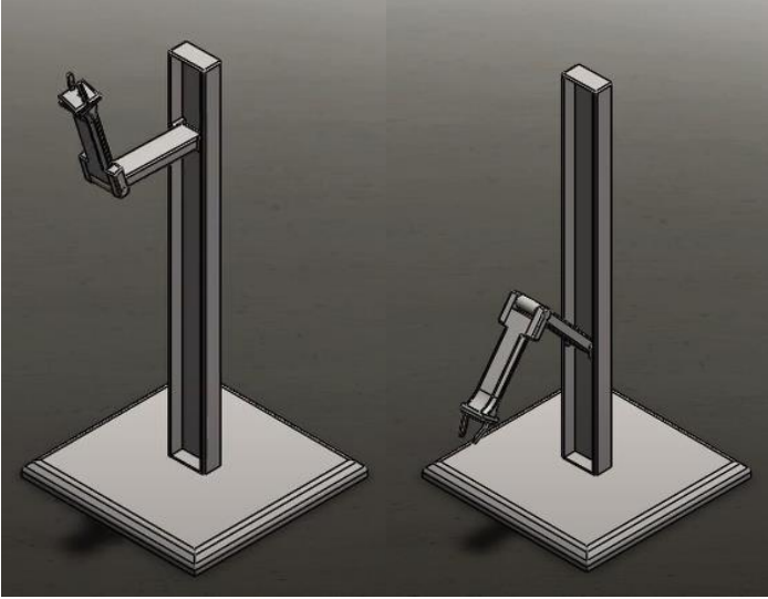
Figure 1. Proposed manipulator
