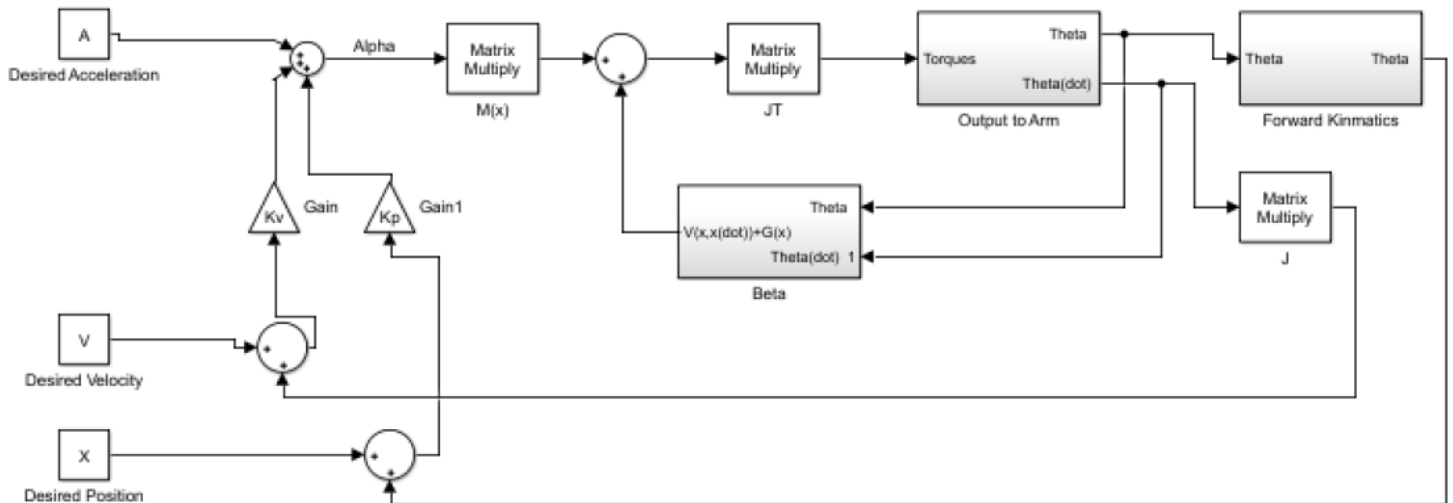
Figure 3. Control Block Diagram
