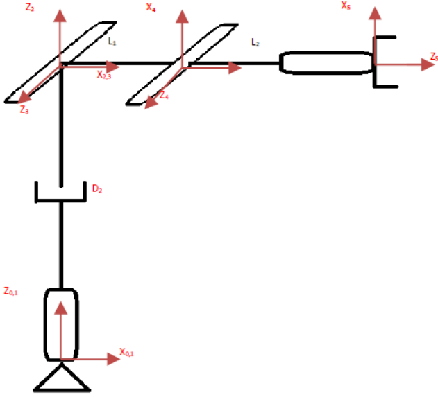
Figure 2. Joint Layout and Frames
